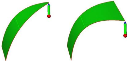
Figure 4. Interactive Skinning
