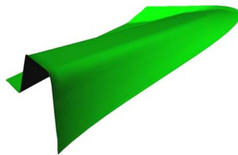
Figure 5. Coons Patch
